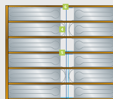
System shown: Modular Heating Panel
